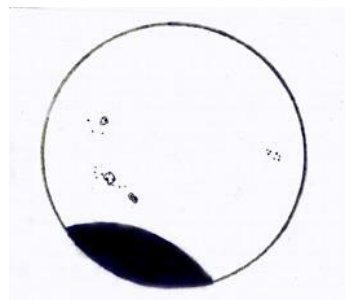
Partial Eclipse
