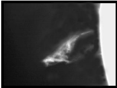
Partial Eclipse
