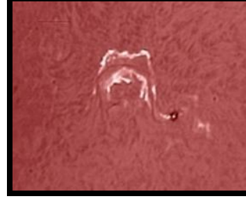
Diamond Ring
