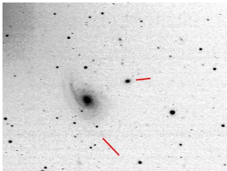
Arp78 - Aries NGC770 & 772
